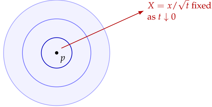
geometry freezes to its curvature model at p
